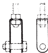
FIG 29-1529 LINK EYE
