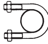
FIG 3BS-1503BS U BOLT ANCHOR BS 3974
