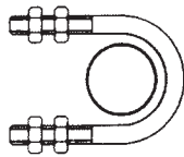
FIG 3A-1503A U BOLT GUIDE (STEEL PIPE)
